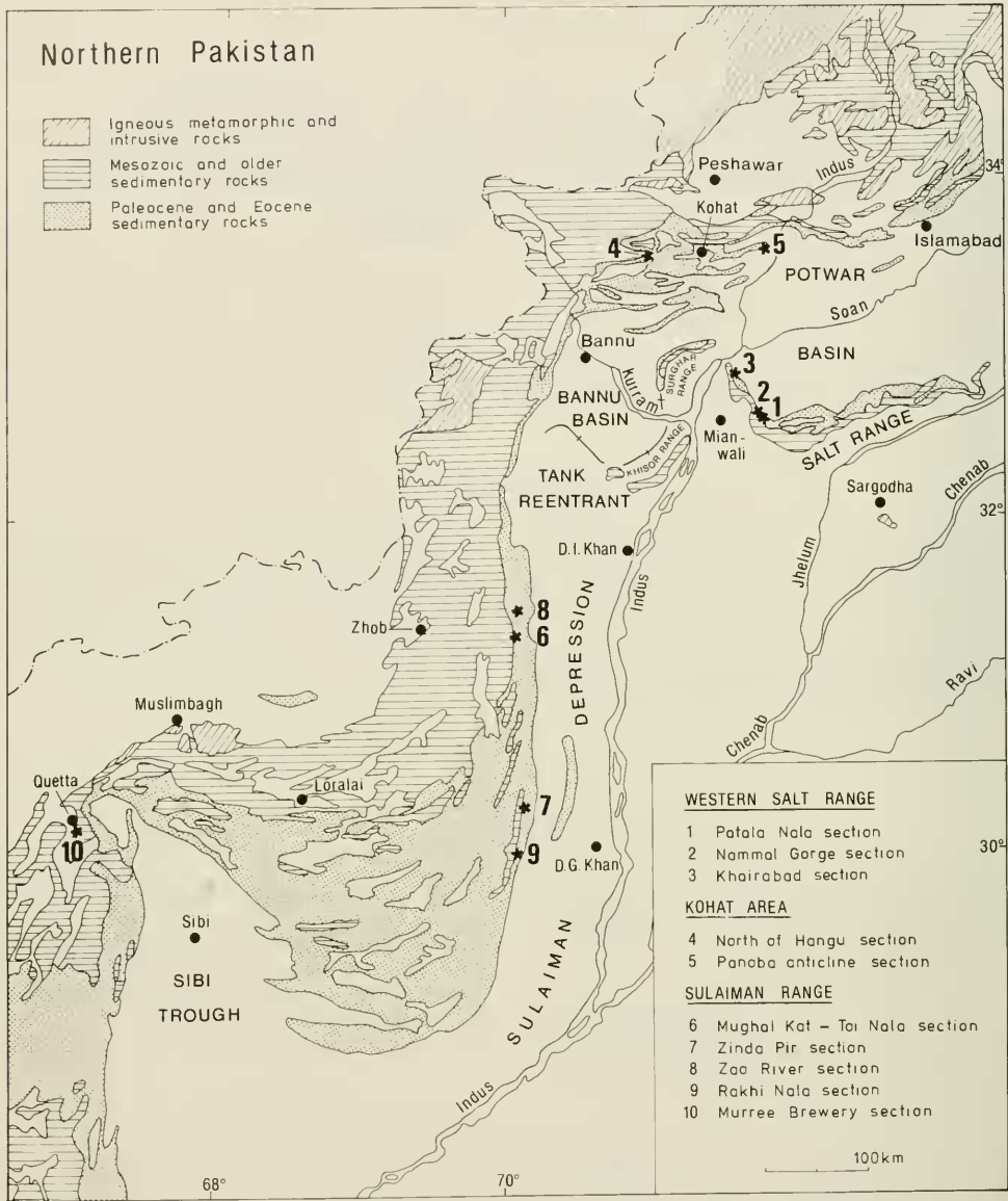
Fig. 1: Location map of investigated sections of the Upper Indus Basin (after EAMES 1952, Geological Map of Pakistan 1:2 000 000 1964, SIIAH 1977 and PORTH & KAMRAN in PORTH & HILAL A. RAZA 1988).
